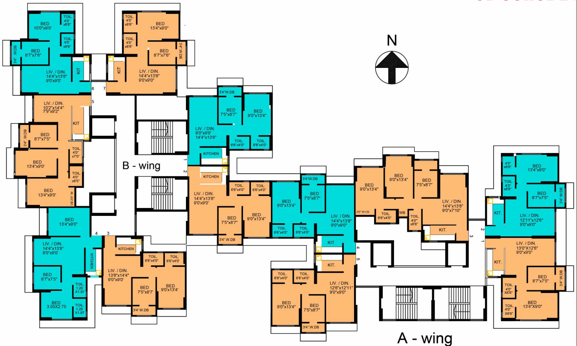
3rd to 6th , 8th to 11th ,13th to 15th Floor Plan.
